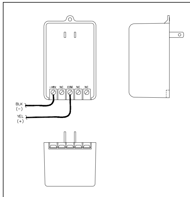
Figure 4. Transformer Details
